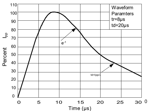
Figure3: Pulse Waveform
