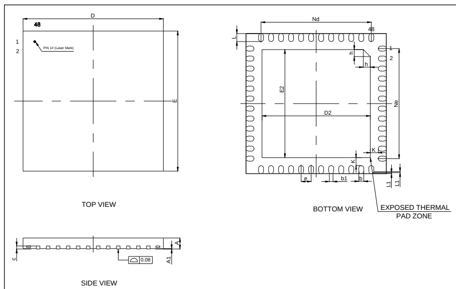
Figure 5-9. QFN48 package outline
