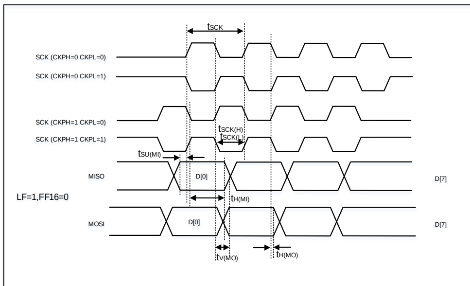
Figure 4-6. SPI timing diagram - master mode
