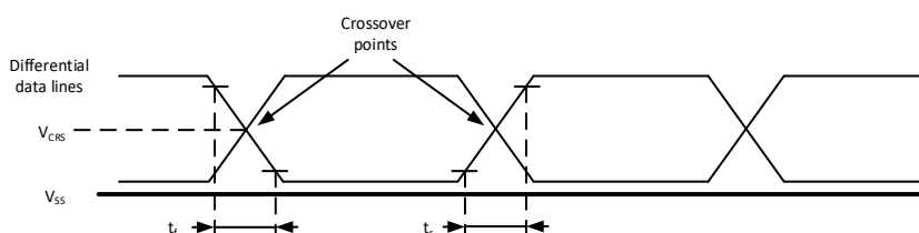
Figure 4-10. USB D timings: definition of data signal rise and fall time
