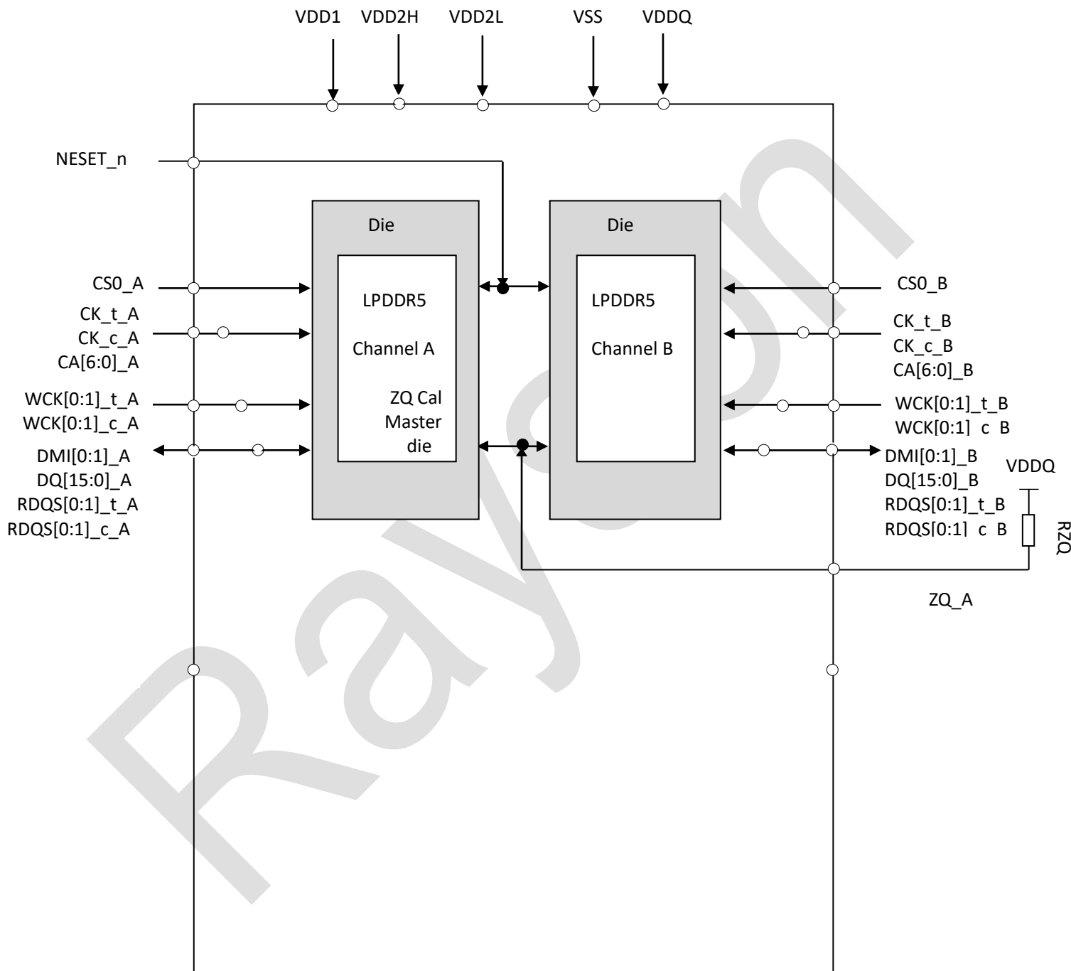
Dual-Die, Dual-Channel Package,Block Diagram
