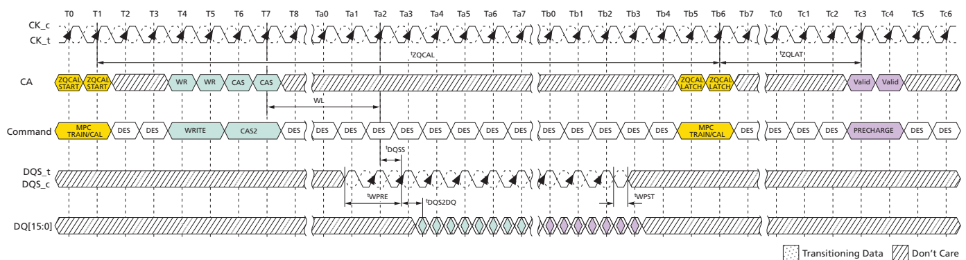
Figure 138: ZQCAL Timing
