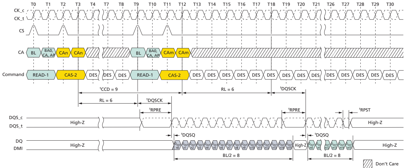
Figure 46: Consecutive READ: t_{CCD} = \text{MIN} + 1 , Preamble = Static, 0.5n\text{CK} Postamble
