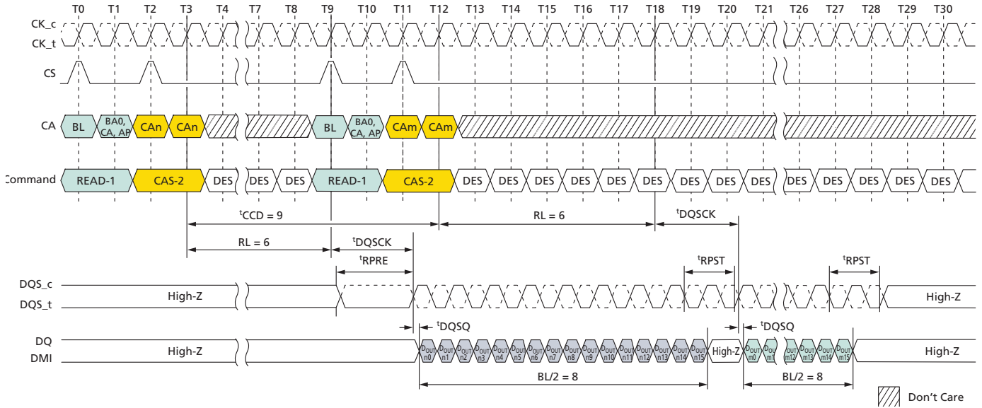
Figure 45: Consecutive READ: t_{CCD} = \text{MIN} + 1 , Preamble = Static, 1.5n\text{CK} Postamble
