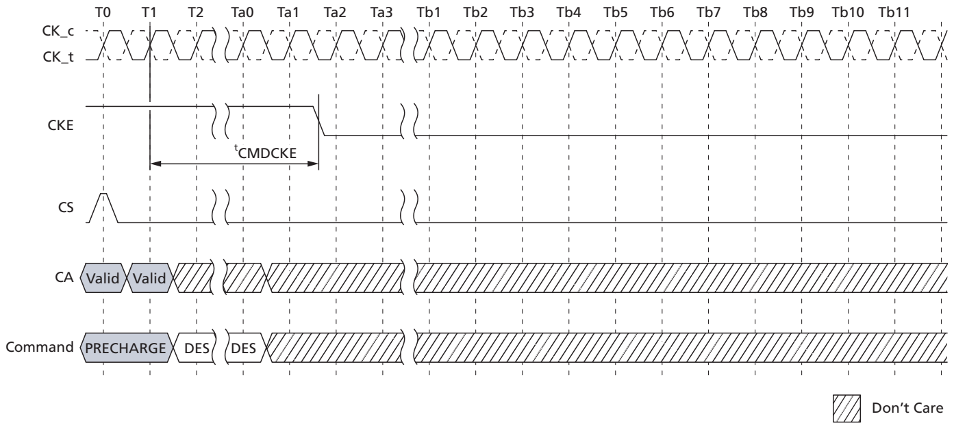
Figure 90: PRECHARGE Command to Power-Down Entry
