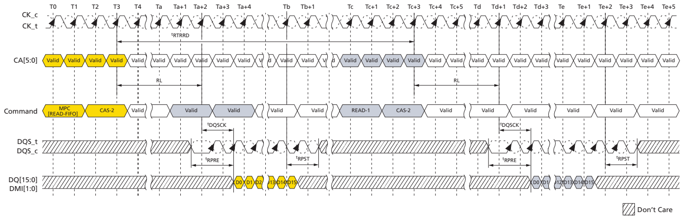
Figure 125: READ-FIFO – t_{\text{RPRE}} = \text{Toggleing} , t_{\text{RPST}} = 1.5n\text{CK}
