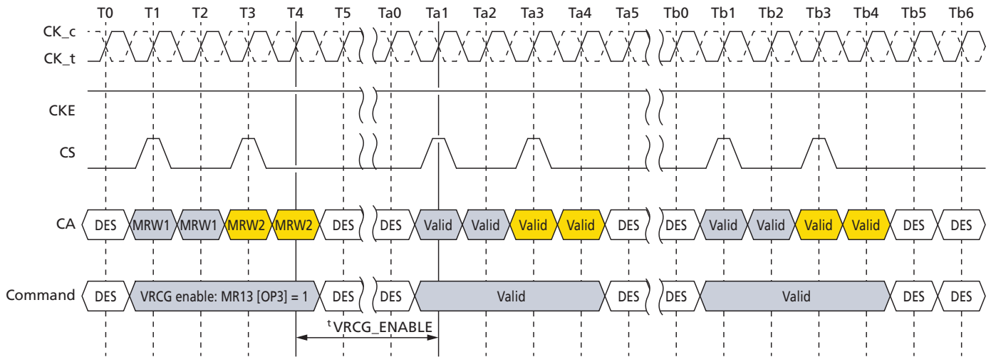
Figure 99: VRCG Enable Timing
